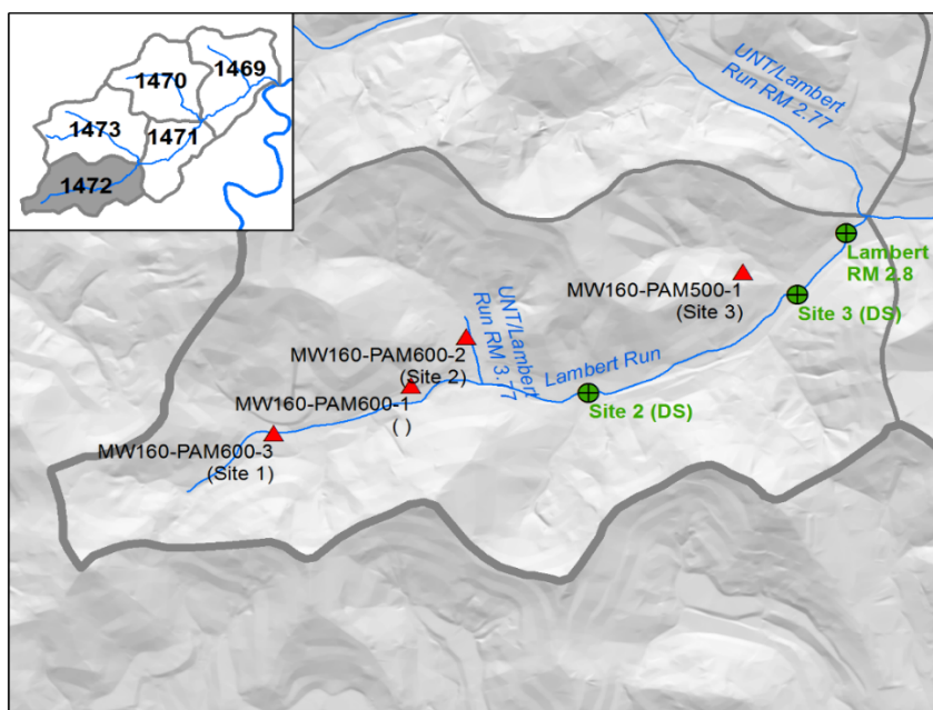
Figure 7: Subwatershed 1472 contains the headwaters of the mainstem of Lambert Run.
