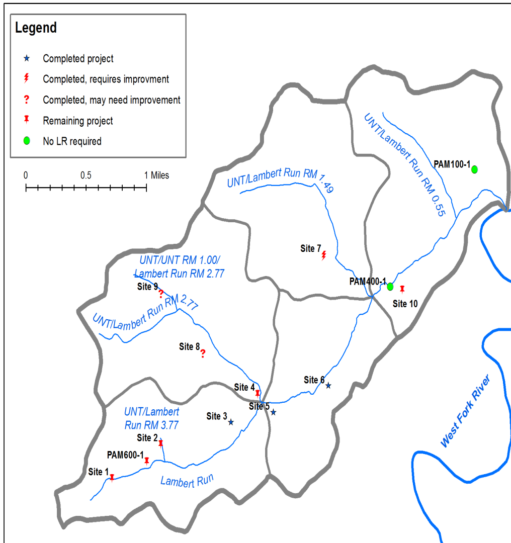
Figure 5: Lambert Run has four tributaries and one tributary to a tributary. Thirteen possible mine drainage sources have been identified, but no work is needed at six of them.
