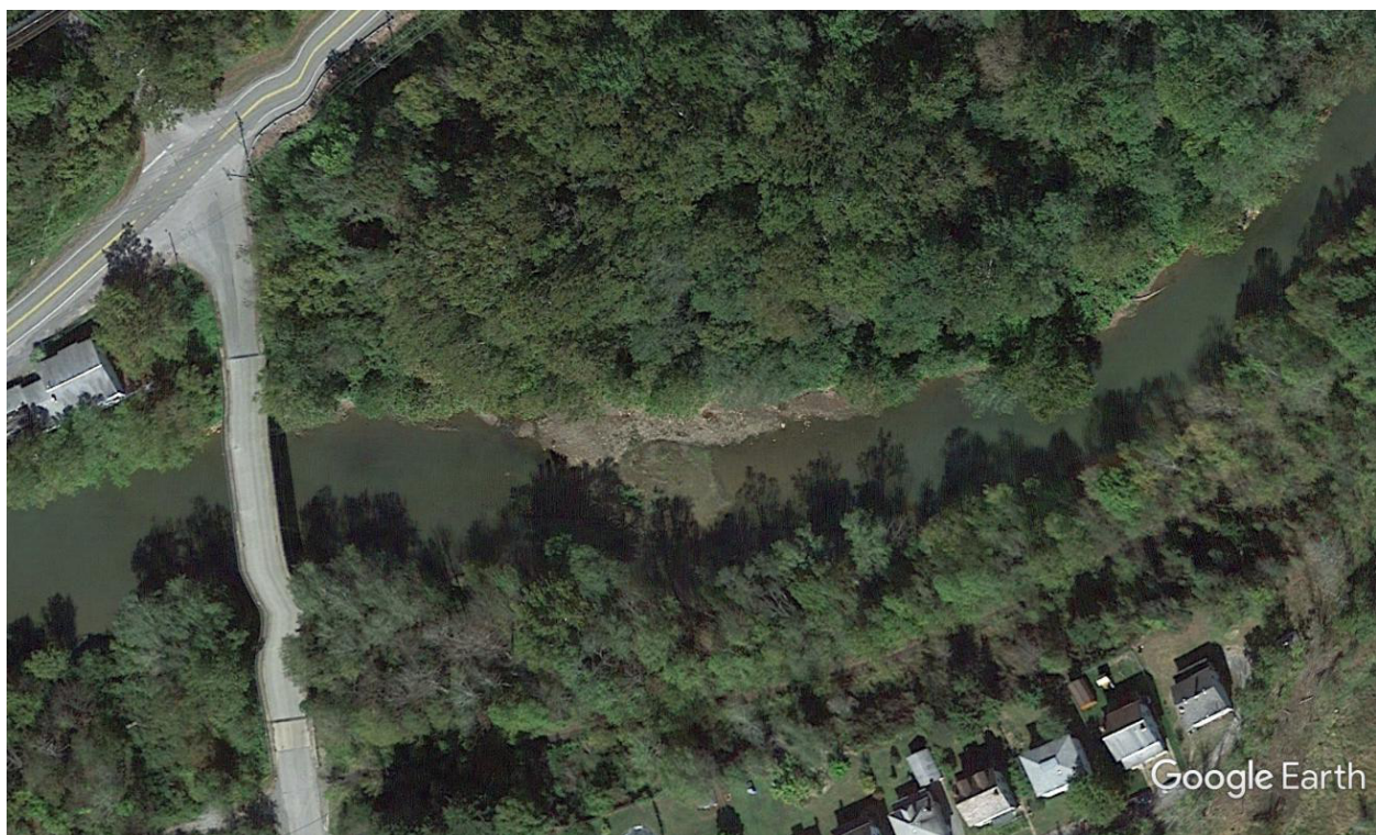
Figure 3: 2016 imagery at the same site shows a delta of sediment below Lambert Run, but relatively clear water.
